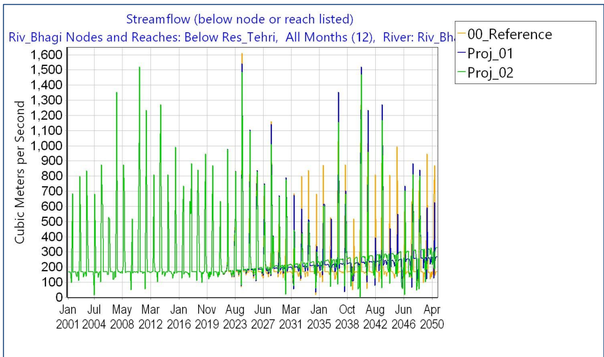
Figure 33. Monthly outflow from Tehri dam under the reference and the two projections.
