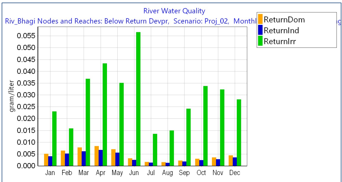
Figure 37. Mean monthly dependency on return flows flowing out of the basin under the reference (top) projections Proj_02 (extreme). Top: 2011-2020 (Reference); bottom 2041-2050 (Proj_02). Note: Y-axis values are concentrations of the virtual tracers. And are identical as fractions. Total for each month is not necessary 1 (=100%) as only reuse of water is presented.
