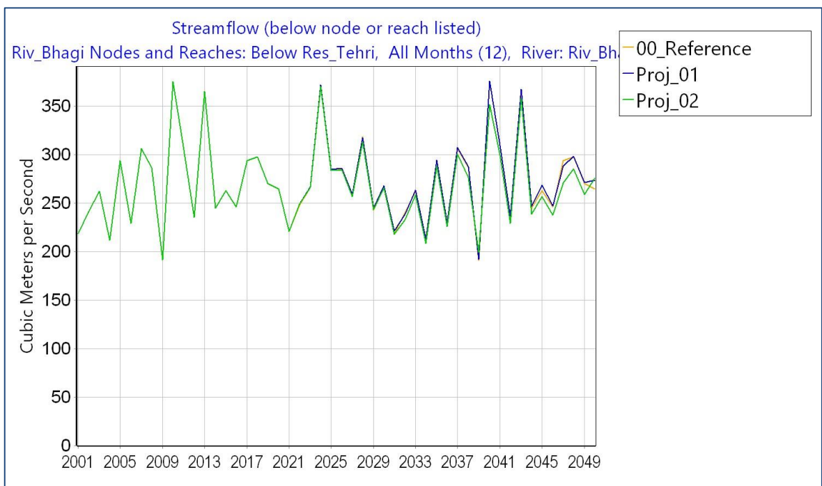
Figure 34. Mean annual outflow from Tehri dam under the reference and the two projections.
