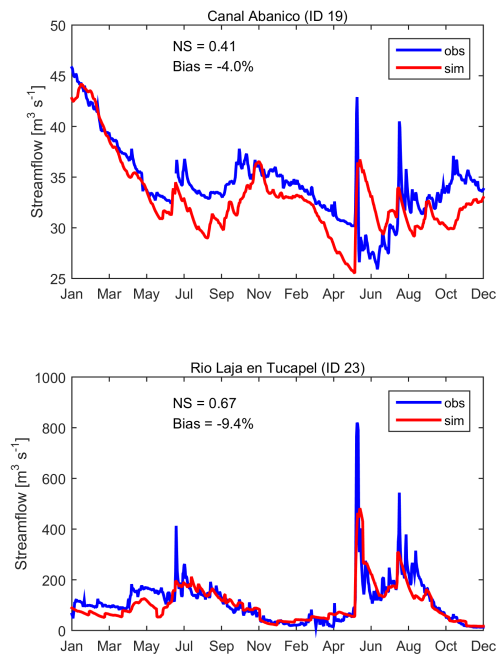
Figure 11. Daily observed vs. SPHY simulated streamflow (period 2007–2008) for the streamflow stations Canal Abanico (ID 19) and Rio Laja en Tucapel (ID 23). The Nash–Sutcliffe (NS) and bias model performance indicators are shown as well.
