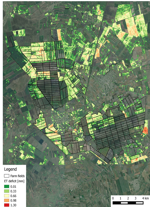
Figure 4. Spatial distribution of evapotranspiration (ET) deficit, as simulated by the SPHY model for a Romanian farm on 03 April 2014. Transparency means no ET deficit.
