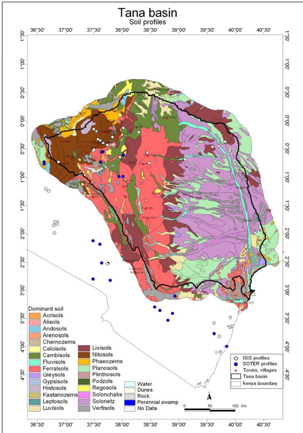
Figure 36: Tana Basin, soil groups and availability of soil profile data
