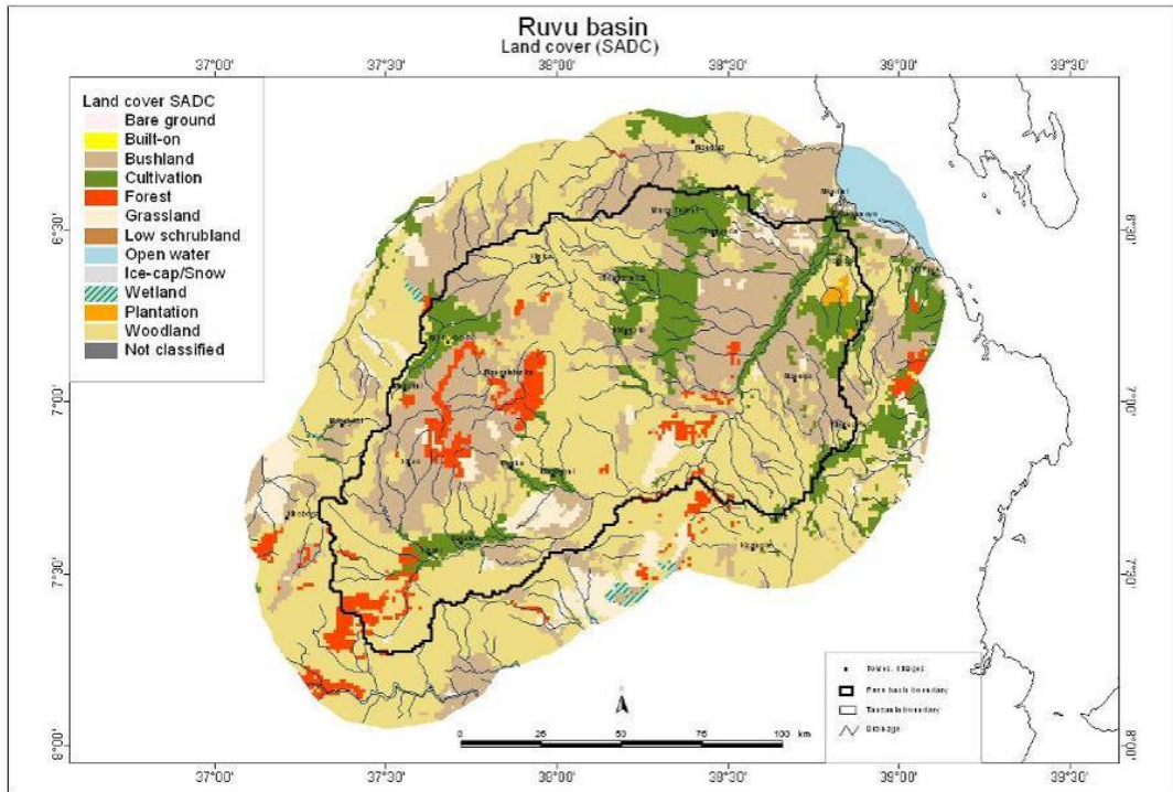
Figure 46: Ruvu Basin, land cover Source: SADC Regional Land Cover Database Project
